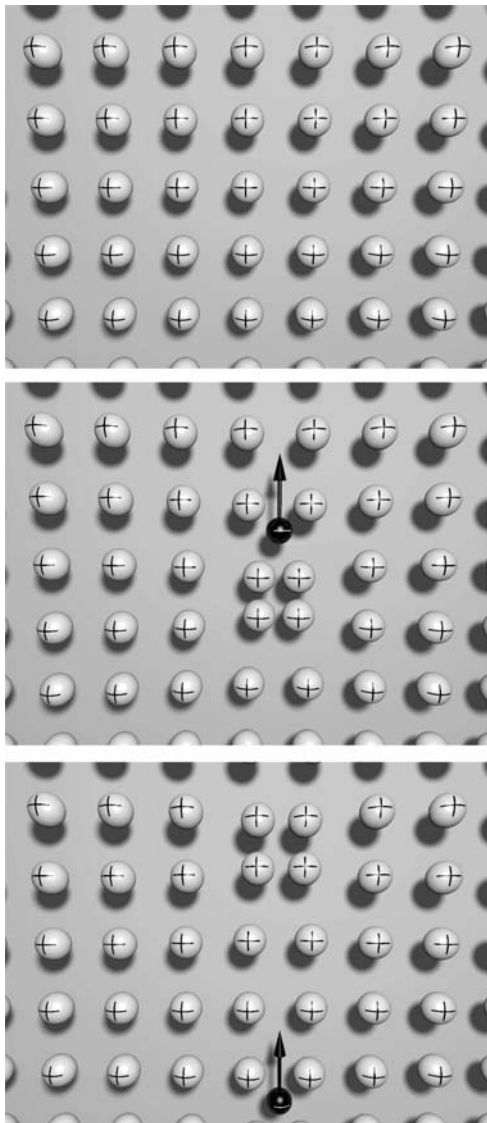
14. The lattice of positively charged ions (top panel). A negatively charged electron in a superconductor distorts the lattice of positively charged ions as it passes through (middle panel). Because the heavy ions take a longer time to respond, there is still an excess positive charge to help the second electron of the Cooper pair travel through (bottom panel)
