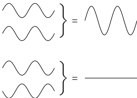
11. Two waves combine (top) with the same phase, resulting in constructive interference, or (bottom) with opposite phase, resulting in destructive interference
